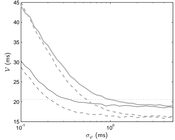
Figure 3. Black lines: as in figure (2). The second simulation included here (thick gray lines) was obtained sampling the synthetic ECG signals at 200 Hz instead of 1000 Hz (broadband 30 \mu\text{V} peak-to-peak noise was still added).
