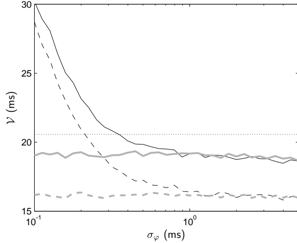
Figure 2. Mean estimates for the \mathcal{V} -index obtained on simulated ECGs for the 8 independent leads of the standard configuration (sketched lines) and the Frank’s orthogonal system (continuous line). The figure refers to the case s_{\vartheta} = 20.6 ms (horizontal dotted line) and two simulations are comprised in the graph: broadband 30 \mu\text{V} peak-to-peak noise added to the synthetic ECGs (black), and no noise added (gray thick lines).
