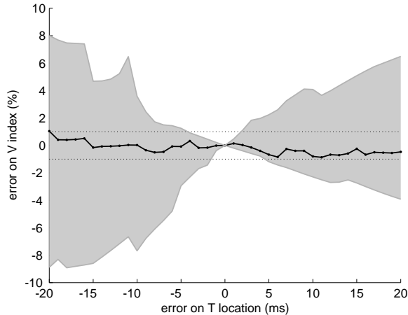
Figure 4. Percent relative error on the estimates of the \mathcal{V} -index. It was evaluated displacing artificially the end of the T wave of a maximal quantity (abscissas). The continuous line reports the mean value obtained on the E-OTH-12-0068-010 THEW database. The gray area includes 90% of the error population (it was drawn between the 5% and the 95% percentiles). The two dotted horizontal lines marks the \pm 1\% values.
